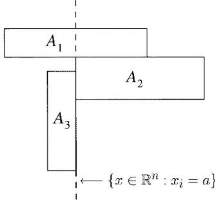
Figure 6.2: separating hyperplane
