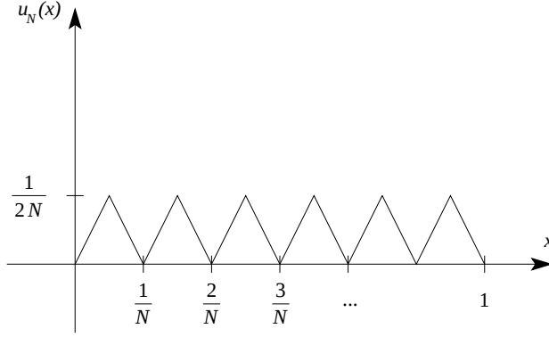
Figure 3.1: minimizing sequence
